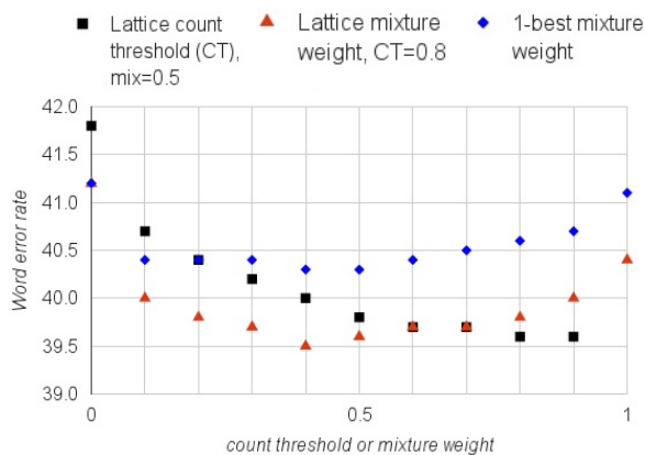
Figure 1: Parameter sweep on the dev set of: (1) count threshold values for fractional counts from lattices, with mixture weight fixed at 0.5; and (2) weights for mixing with the baseline model for both lattice and one-best methods, with fractional count thresholding fixed at 0.8.
