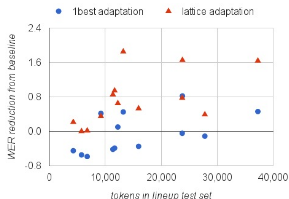
Figure 2: WER reduction vs. number of tokens in the test set, for both one-best and lattice-based adaptation for each of the lineups examined.
