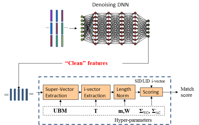
Figure 2: Hybrid denoising DNN i-vector system
