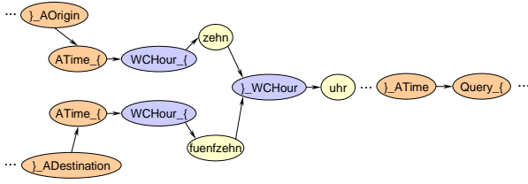
Figure 1: Snippet of exemplary flat lattice with nodes marking beginnings (..._) and endings (_...) of semantic units.
