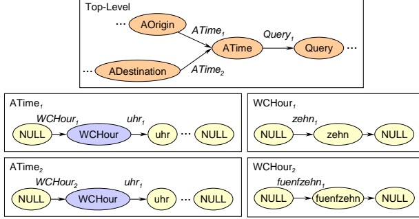
Figure 2: Snippet of lattice hierarchy corresponding to flat lattice of Figure 1.
