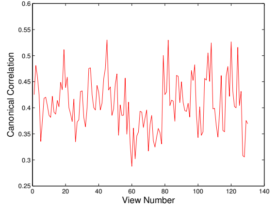
Figure 1: Canonical Correlation of LLD based views against the physical load labels (Low/High). The views are sorted lexicographically with respect to the LLD names
