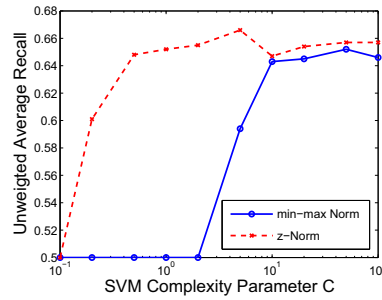
Figure 4: Performance of SVM with RBF Kernel on multi view LFDA selected features.
