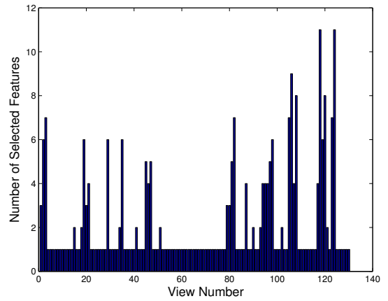
Figure 2: The number of selected features with CFS per view. The views are sorted lexicographically with respect to the LLD names
