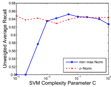
Figure 3: Performance of SVM with Linear Kernel on multi view LFDA selected features.
