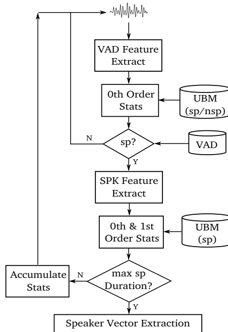
Figure 1: Speaker vector extraction in the EML Online speaker diarization system.
