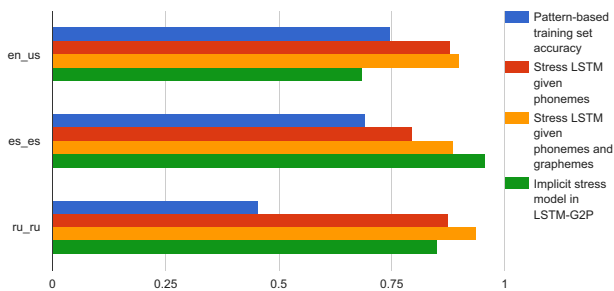
Figure 1: Stress model accuracies for selected languages.
