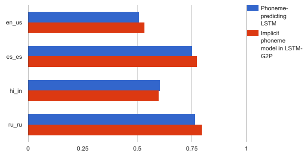
Figure 2: Phoneme model accuracies for selected languages.
