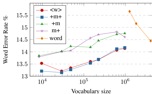
Figure 4: Comparison of vocabulary size vs Word Error Rate for each style of marker.
