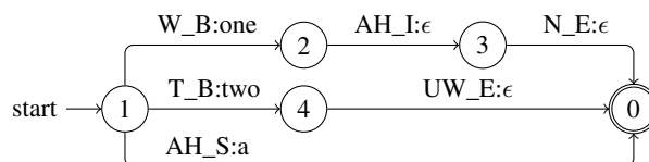
Figure 2: Example of the \$complete FST for the lexicon ‘one’ ( WAHN ), ‘two’ ( TUW ) and ‘a’ ( AH ), with position ( _B : begin, _E : end, _I : internal, _S :single) marked.
