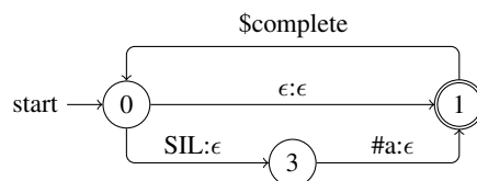
Figure 1: Prototype \mathcal{L} -FST for a standard word lexicon. Each arc is labeled with its corresponding input:output symbols. The \$ -syntax indicates the location for replacement with a second FST named x .
