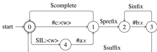
Figure 3: Prototype subword L-FST, specifically for the <w> style tags. For other markers the prototype is the same except that all <w> tags are replaced by \epsilon .
