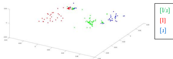
Figure 3. PCA visualization of the activations of the 4th hidden layer to input /l/, /r/, and the ambiguous sounds in the ambR model.
