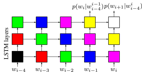
Figure 1: Jitter n -gram: example of a 3-layer, 5-gram, recurrent NNLM with a jitter of 2. Layers are unfolded along the word sequence, and blocks with the same color are evaluated in parallel.
