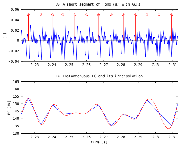
Figure 1: An example of instantaneous F0 estimation for a short segment of long /a/.
