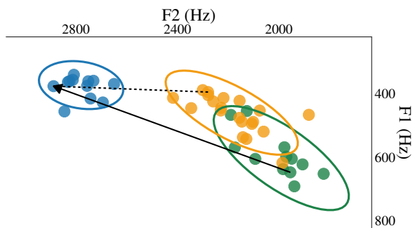
Figure 4: Realizations of ⟨-ä-⟩ by user f04 during task 1 ( base ) and task 4 ( map ) relative to Mirabella’s productions of [ɛ:] during task 4 ( map ). The arrows illustrate the Euclidean distance to the target word ähnlich as an example. The ellipses indicate the 95 % confidence interval.
