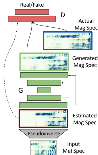
Figure 2: Adversarial Vocoder Model : The generator performs an image-to-image translation from the estimated magnitude spectrogram to the actual magnitude spectrogram guided by an adversarial loss from the discriminator and the L_1 distance between the generated and actual magnitude spectrogram
