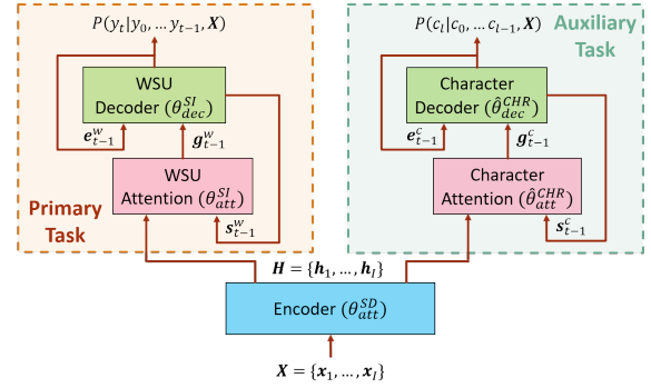
Figure 3: MTL speaker adaptation of AED model for E2E ASR.
