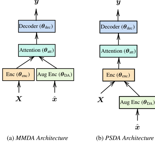
Figure 1: MMDA and PSDA . \mathbf{X} is the original speech, \hat{\mathbf{x}} is the text-based augmenting input, and \mathbf{y} is an output character sequence. \theta_{enc} , \theta_{att} , \theta_{dec} , \theta_{DA} , are the parameters corresponding to the encoder, attention, decoder, and data-augmenting encoder respectively
