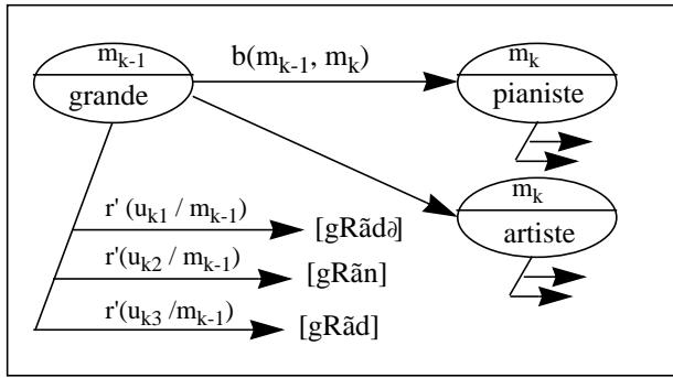
Figure 1: Illustration of an example of (W,P) model.
