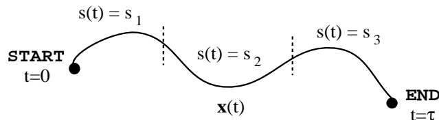
Figure 1: Two variables—one continuous ( \mathbf{x} ), one discrete ( s )—evolve jointly in time. The trace of s partitions the curve of \mathbf{x} into different segments whose boundaries occur where s changes value.
