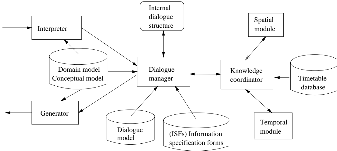
Figure 1: An overview of the linlin system
