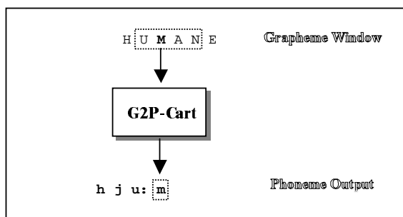
Figure 1. Schematic diagram of the run-time G2P-Cart
