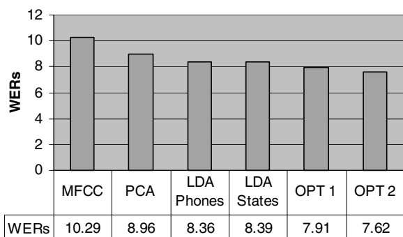
Figure 1: Word error rates for the DARPA Resource Management Corpus obtained using various feature generation schemes. LDA Phone and LDA State refer to LDA obtained using phone classes and state classes, respectively. OPT 1 is the proposed method derived by maximizing the normalized acoustic likelihood over all training frames, and OPT2 is the proposed method derived by maximizing the normalized acoustic likelihood only for misclassified frames of training data.
