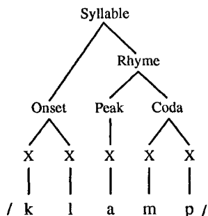
Figure 2. Phonological structure of the monosyllabic word 'clap'. Redrawn from [4].
