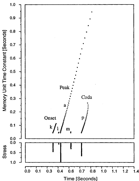
Figure 3. Rhythmogram of the monosyllabic word 'clap'.
