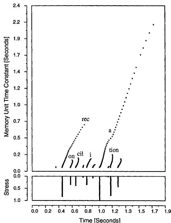
Figure 5. Rhythmogram of the utterance 'reconciliation'.
