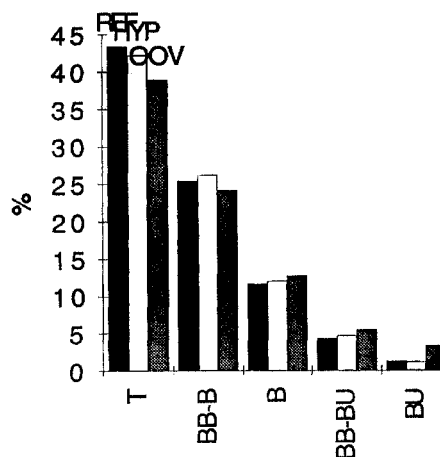
Figure 4: Overall rates of language model transition types. The left-hand bars represent rate within non-OOV reference utterances. Middle bars represent rate within the corresponding decoder output. Right-hand bars represent rate within the decoder output of OOV utterances.
