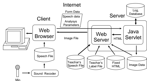
Figure 1: Block diagram of the learning system.
