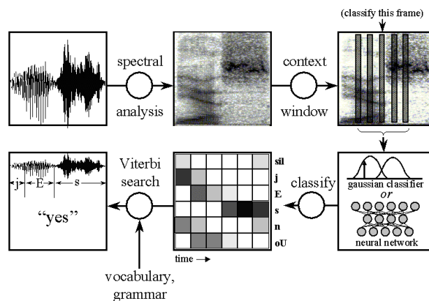
Figure 1. Illustration of the recognition process using the HMM/ANN hybrid architecture in the CSLU Toolkit.
