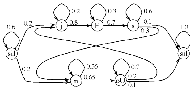
Figure 2. Illustration of a state sequence in an HMM or HMM/ANN hybrid system.
