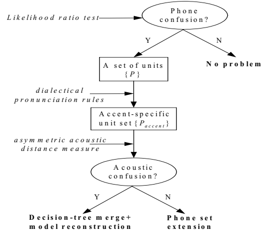
Fig. 3: State-transition charts of modeling phonetic and acoustic confusions in accented speech.
