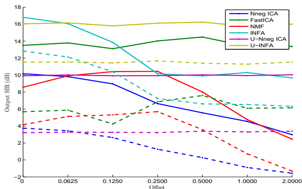
Fig. 2. Output SIR vs. offset for a mixing matrix with twice as many observations as sources in the presence of additive noise with an input SNR of 19 dB. ( n_o = 6, n_s = 3 ). Solid lines show average performance. Dashed lines show the worst SNR out of the three recovered sources.
