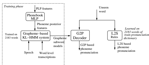
Figure 3: Illustration of pronunciation model generation using G2P and L2S approaches
