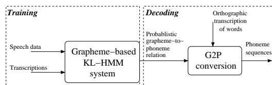
Figure 1: Block diagram of the proposed two phase G2P conversion approach.
