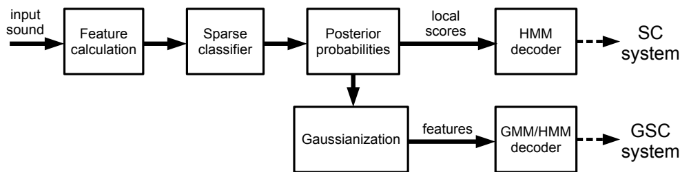
Figure 1: Block diagram of the SC baseline system, which uses posteriors as local scores, and the GSC system, in which posteriors are treated as features and imported to a GMM/HMM decoder.
