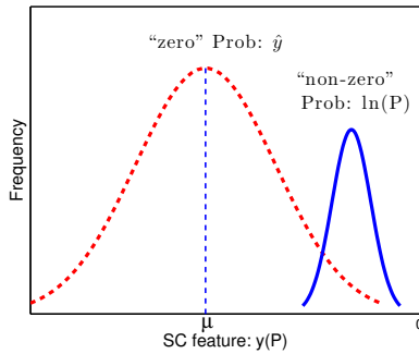
Figure 2: A schematic diagram of two distributions generated by two conditions in Eq. 4.
