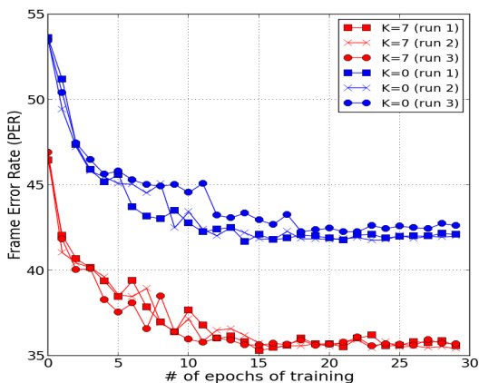
Figure 5: Frame Error Rate (FER) of DART on WSJ using DNNs with six hidden layers of 2000 units each. Each model used \pm 7 frames of context. The DNN's were trained to predict \pm 7 frames of context for the multi-frame models ( K = 7 ) and only the central frame for the non-multi-frame models ( K = 0 ).
