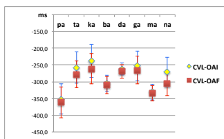
Figure 3: Delay between the first visual event (for the closing phase) and the first auditory event (for the opening phase) in isolated /Ca/. Same display as in Fig. 2.
