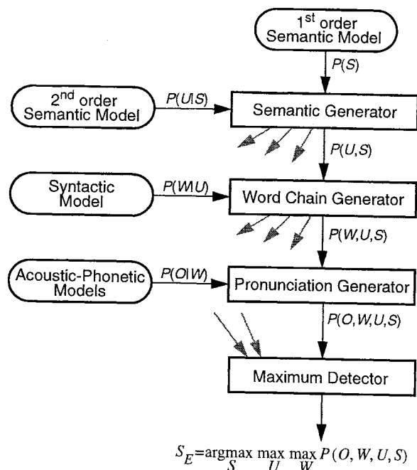
Figure 1: Search for the most probable semantic content by generating hypotheses in a 'top-down' strategy
