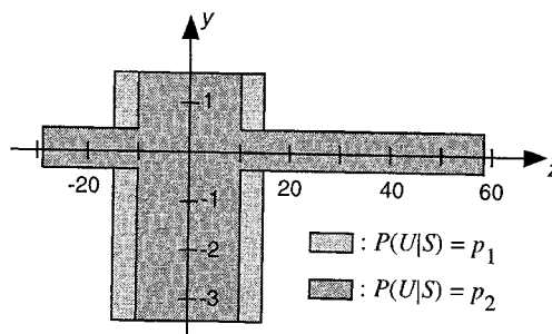
Figure 3: Discrete 2 nd order semantic model
