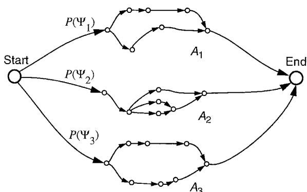
Figure 5: Example language model, consisting of three paralleled automata A_1, A_2 and A_3
