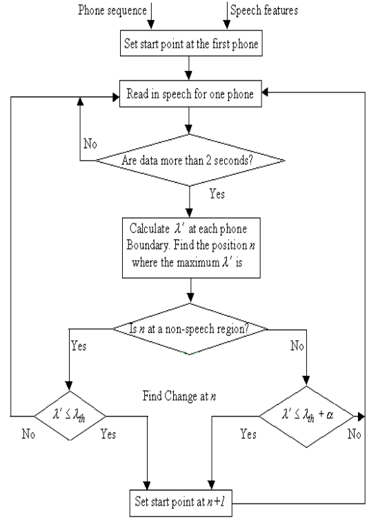
Figure 2. Speaker Change Detection Flow-chart.
