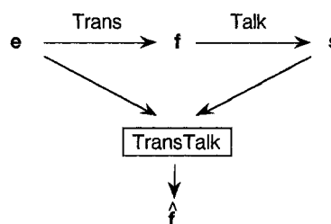
Figure 1: TransTalk's underlying model. Starting from an English sentence e , the translator mentally formulates its French translation f , then produces its acoustic rendering s . The system's aim is to find \hat{f} = \operatorname{argmax}_f p(f|e, s) , or equivalently, from Bayes's formula, \hat{f} = \operatorname{argmax}_f p(s|e, f) \cdot p(f|e) . By neglecting the influence of e on s once f is known, we can take \hat{f} = \operatorname{argmax}_f p(s|f) \cdot p(f|e) .
