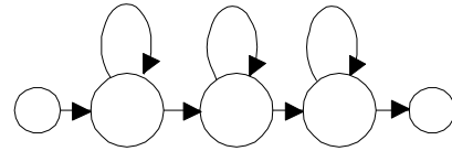
Figure 3: Three-state left-to-right HMM architecture.
