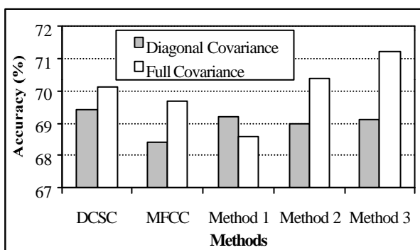
Figure 3 Monophone results of different methods with diagonal and full covariance mixtures.
