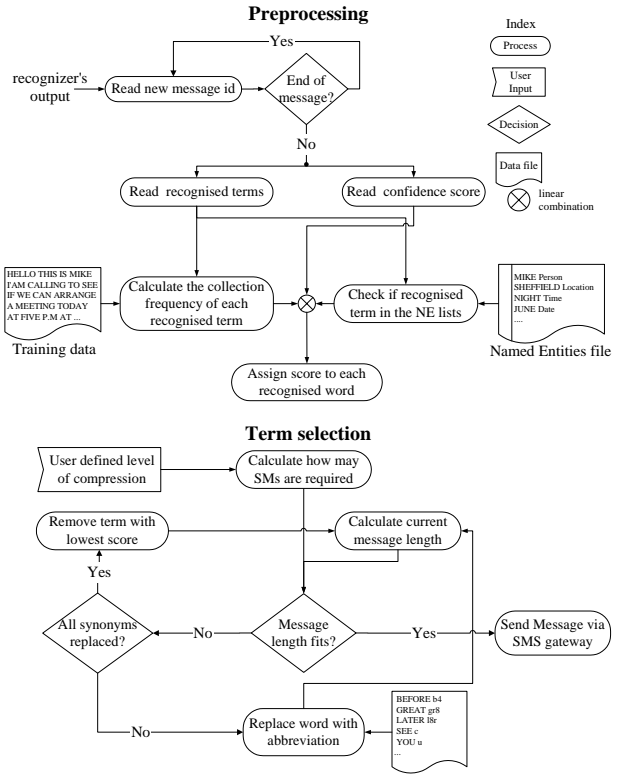
Figure 1: A schematic outline of the mechanism that summarizes the decoder’s output using a combination of statistics and prior knowledge.
