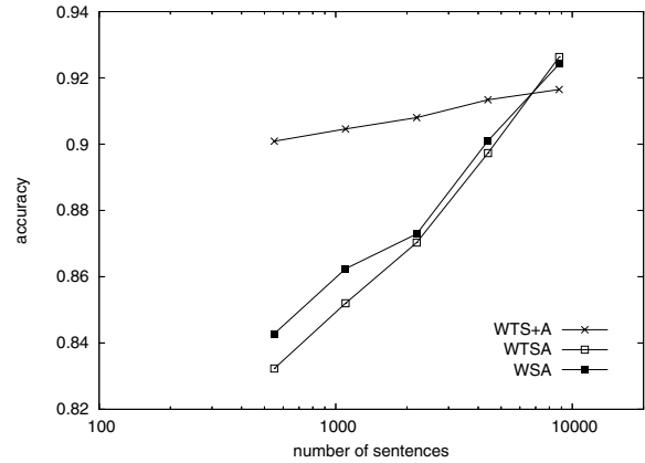
Figure 2: Learning curve for accents. Solid lines represent approximate accuracy for accents : \langle w, s, a \rangle | \langle w, s \rangle .
