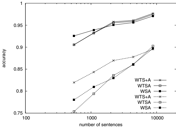
Figure 1: Learning curve for phonemes and accents. Solid lines represent accuracy of \langle w, s \rangle as a reference. Dotted lines represent accuracy of \langle w, s, a \rangle .
