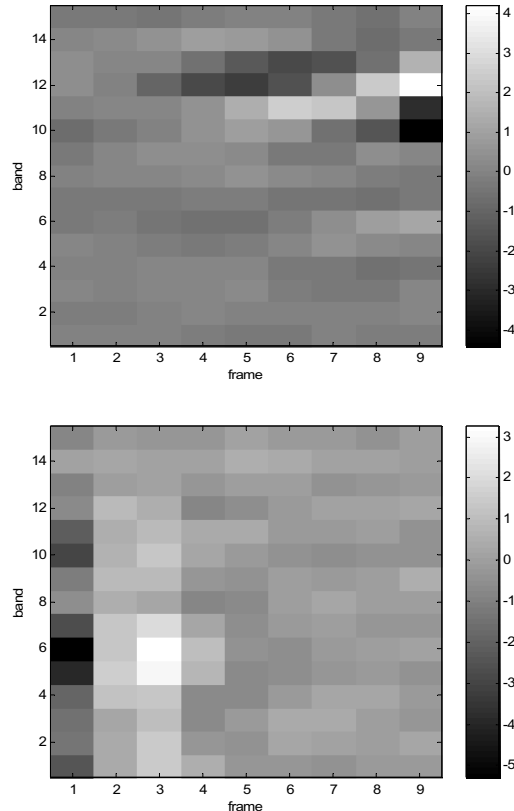
Figure 2: Illustration of the pattern corresponding to the weights connecting to a certain hidden node in the first
