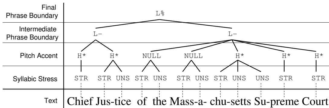
Figure 1: A prosodic tree derived from sequential ToBI transcripts and syllable segmentation of the BURNC [8]. The four tiers of the tree represent prosodic units on increasingly large time-scales, each with a unique linguistic meaning. The ASCII representation of the top three tiers would be TOP (L% (L- (H* H*) L- (NULL NULL H* H* H*) ) ). The text is not part of the tree structure but is included here for illustration. Note that the pitch accents’ bounds match the foot rather than the word, following [5].
