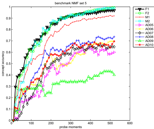
Figure 4: NMF, on the full training set F1+F2+M1+M2.
