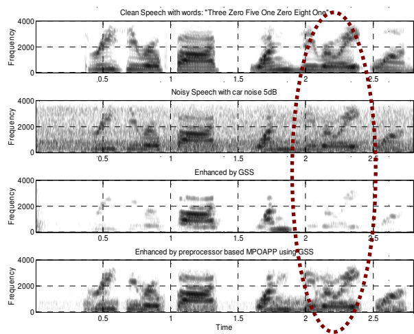
Figure 6. Spectrograms showing (a) clean speech with words “Three Zero Five One Zero Eight One”, (b) the same speech with 5dB car noise, (c) the noisy speech after enhanced by GSS (d) the noisy speech after MPO-APP enhancement using GSS
