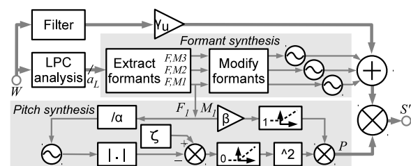
Figure 1: Block diagram of reconstruction mechanism.
