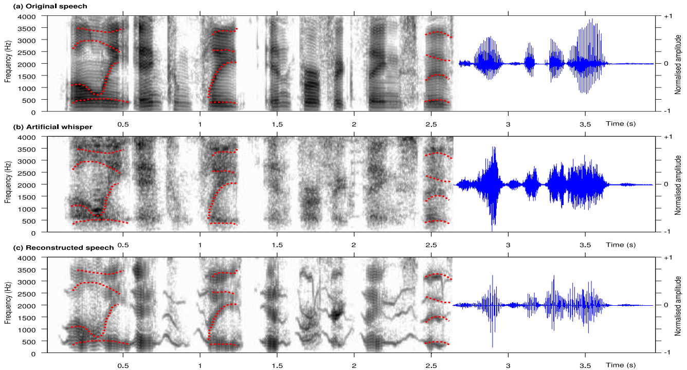
Figure 3: Combined spectrogram/waveform plot for TIMIT utterance sil154 showing original speech S , artificial whisper W and reconstructed speech S' from top to bottom respectively. Manually tracked formants have been overlaid for three phonemes.
