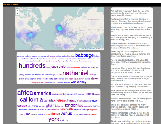
Figure 1: User interface
