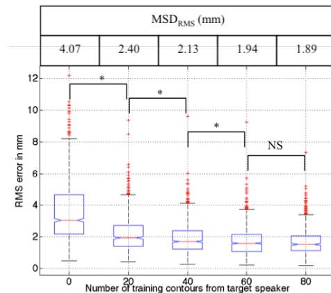
Figure 4: Performance obtained for the speaker-independent experiments as a function of the amount of training images of the target speaker
