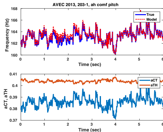
Figure 4: True and model-generated fundamental frequency (top) and inferred CT and TA muscle activations (bottom).
