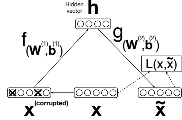
Figure 2: Denoising autoencoder architecture. An input vector \mathbf{x} is stochastically corrupted to obtain \mathbf{x}^{(\text{corrupted})} , then mapped to the latent space \mathbf{h} to extract the reconstructed vector \tilde{\mathbf{x}} . The reconstruction error is evaluated with the loss function L .
