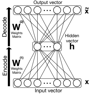
Figure 1: Illustration of the autoencoder model with an input features layer, one hidden layer and the output units. For readability, biases are omitted here.
