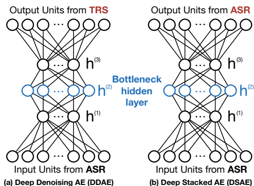
Figure 3: Illustration of the proposed bottleneck features (b) and a deep denoising autoencoder (DDAE) (a).
