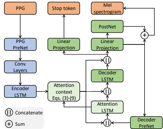
Figure 2: PPG-to-Mel conversion model.
