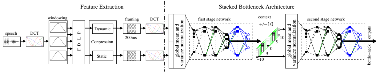
Figure 1: Block diagram of Stacked Bottleneck feature extraction with FDLP front-end.
