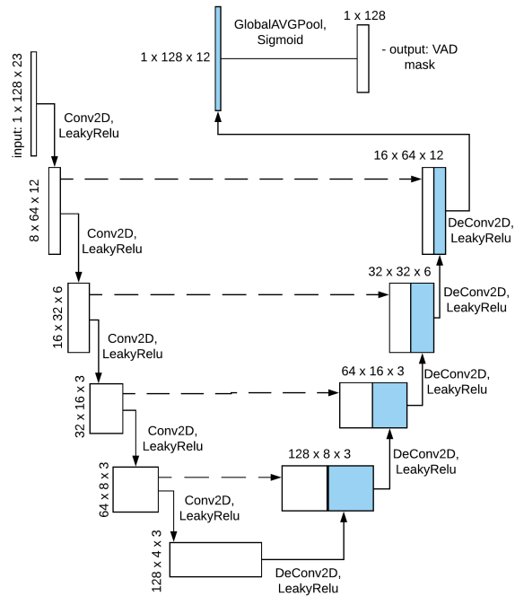
Figure 1: U-net based VAD architecture
