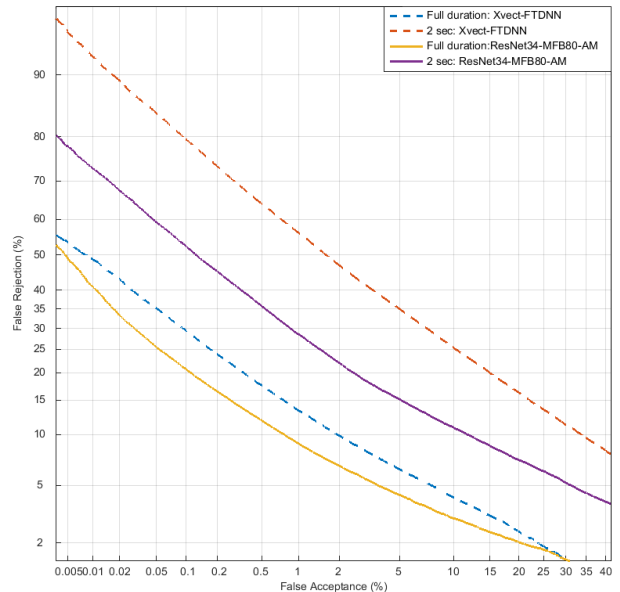
Figure 2: DET curves of Xvect-FTDNN-TrainData-I and ResNet34-MFB80-AM-TrainData-I embedding extractors for full and 2 sec duration of test waveforms from VOiCES (eval set).
