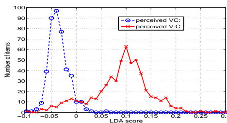
Figure 2: Histogram of LDA score using all features
