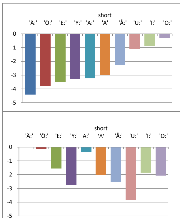
Figure 5: Difference in time between session two and one. Top plot: International subjects (sorted), Bottom plot: Swedish subjects
